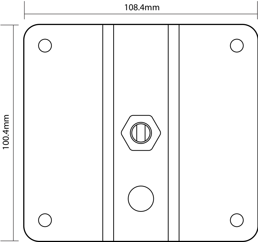
Wall Plate
