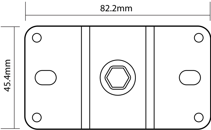
Speaker Plate*
